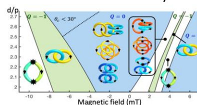
Fig. 3.8. Phase diagrams of stability of solitons phases under confinement in a thin film of thickness d for a chiral colloidal LC with helical pitch p , explored via tuning magnetic field.
