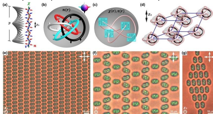
Fig.3.7. Topology & crystals of heliknotons. (a) Field comprising a triad of orthonormal \mathbf{n}(\mathbf{r}) , \mathbf{x}(\mathbf{r}) & \mathbf{\tau}(\mathbf{r}) . (b) Preimages in the smoothly vectorized \mathbf{n}(\mathbf{r}) of a heliknoton coloured according to their orientations on S^2 (inset). (c) Knotted skyrmion structure in \mathbf{n}(\mathbf{r}) co-located with knots of vortex lines in \mathbf{x}(\mathbf{r}) and \mathbf{\tau}(\mathbf{r}) . Gray isosurfaces in (b,c) show regions of distorted helical state. (d) Primitive cell of a triclinic crystal; isosurfaces of distorted helical background are co-located with red vortex knots black/white & preimages of \mathbf{n}(\mathbf{r}) . (e,g) closed & (f) open heliknoton crystal lattices.
